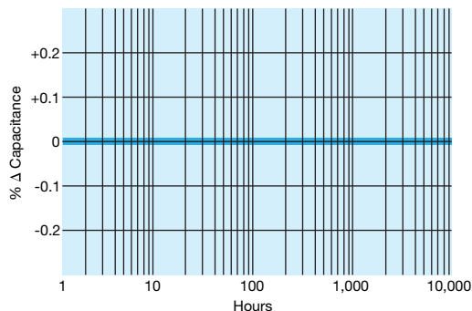
Aging Rate
