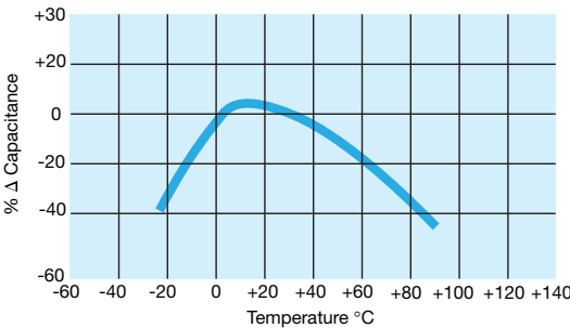
Temperature Coefficient
