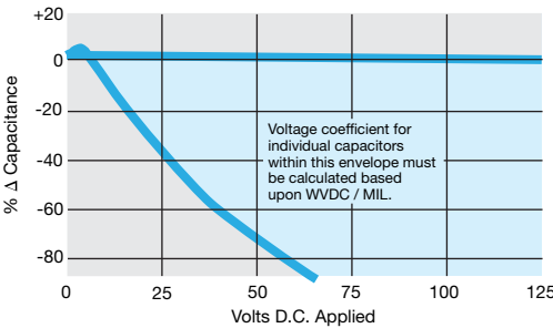
Voltage Coefficient
