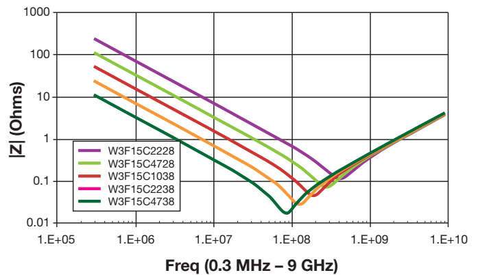
IMPEDANCE 1206 – 50V
