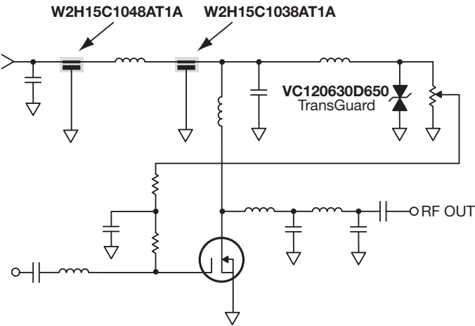
PA Filtering
