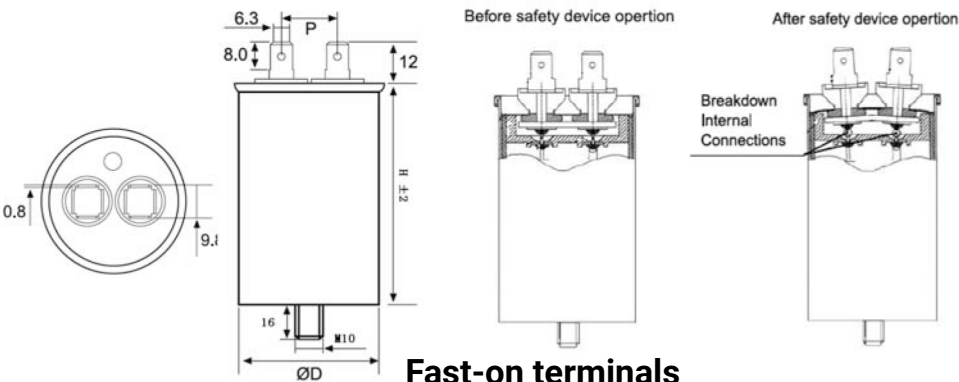
Fast-on terminals
