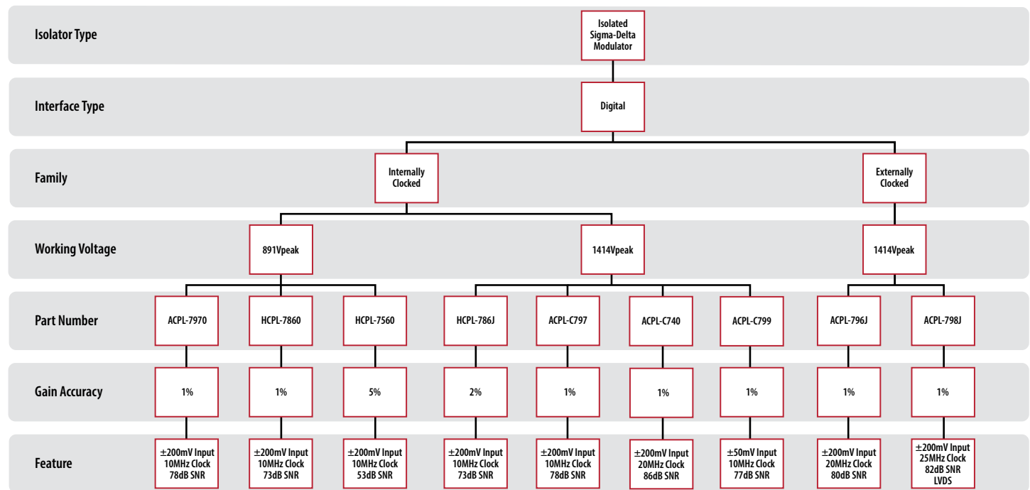
Isolated Sigma-Delta Modulator Product Tree
