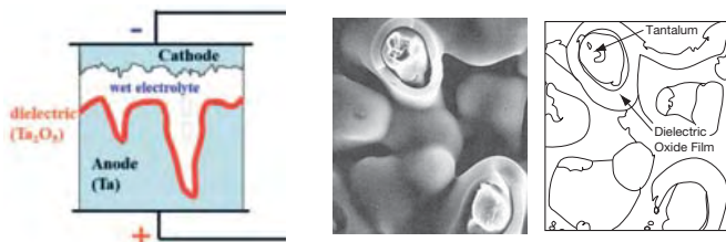
Figure 1 a. Basic Tantalum Wet Electrolytic Capacitor System
