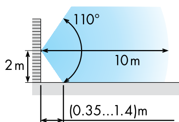
Detection area (side and plan view)
